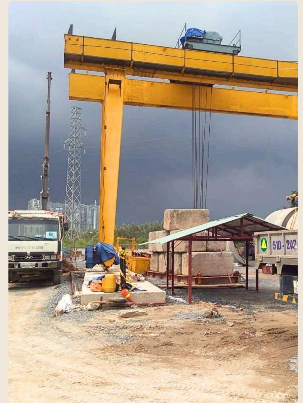
Double Girder Gantry Range: 1000 kg to 200000kg
